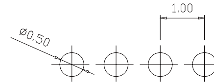
Recommended PCB Layout (PCB TOLERANCE \pm 0.05 )
